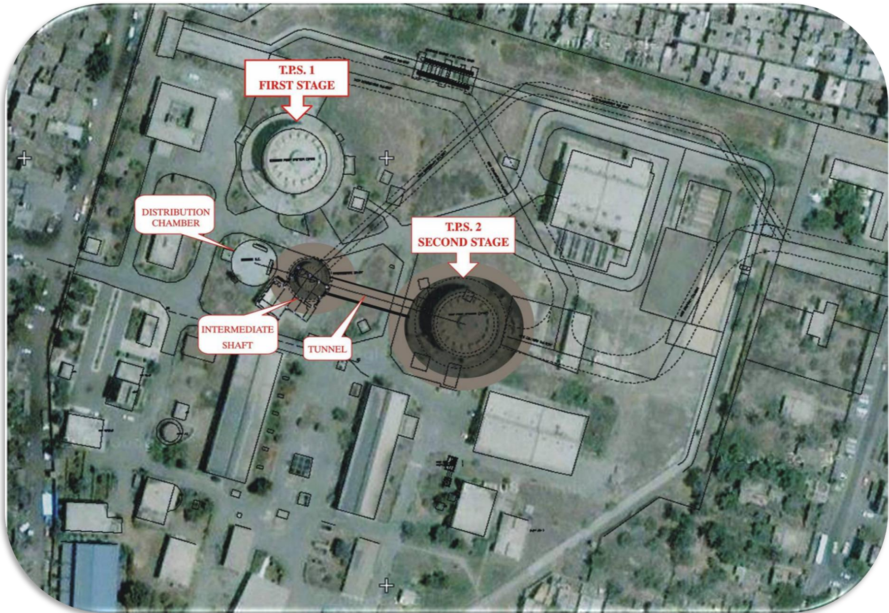
LAYOUT PLAN FOR THE NEW PROJECT STAGE
